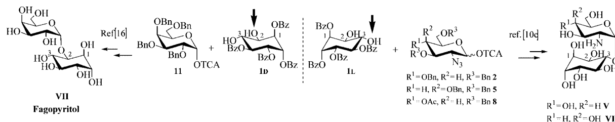
Figure 2. Regioselective reactions of D - and L-chiro inositol acceptors.
