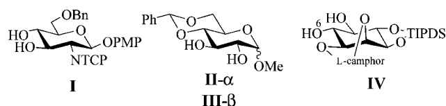
Figure 1. Acceptors that have shown good regioselectivities in glycosylation reactions.
