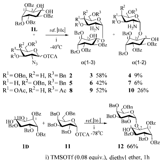
Scheme 1. Reaction of 1L with 2 , 5 and 8 and 1D with 11 .
